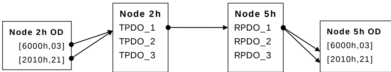
Figure 2: PDO Linking
