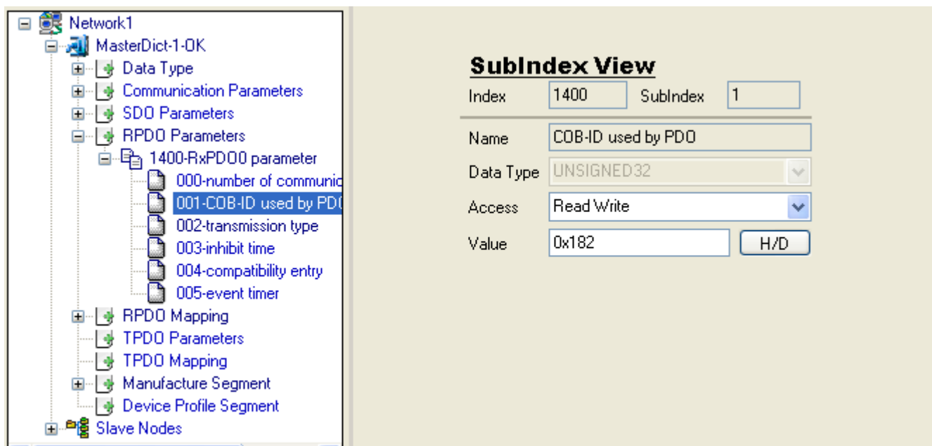
Figure 23: PDO Configuration
